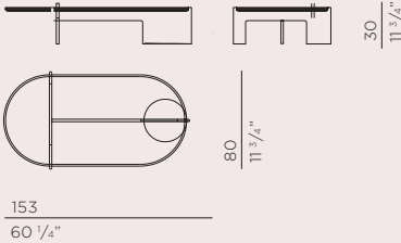
PREST6 oval low table with top 75x150 H30
