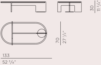
PREST5 oval low table with top 65x130 H30
