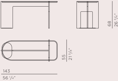
PREST8 console with top 50x140 H68
