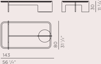
PREST4 rectangular low table with top 75x140 H30
